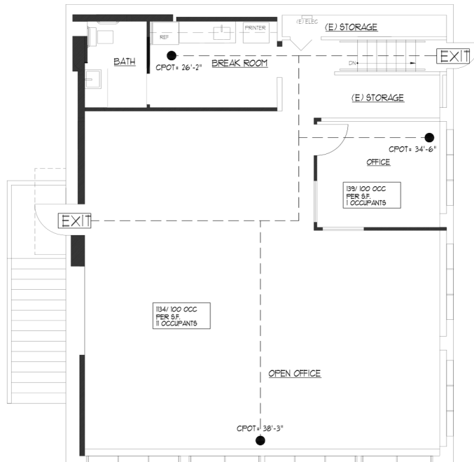
UPPER FLOOR EXITING PLAN (EXISTING EXITS - NO CHANGES) 1/4"=1'-0"
